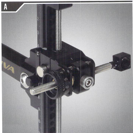
A UPGRADED WITH GROOVED TWIN RAIL SYSTEM
