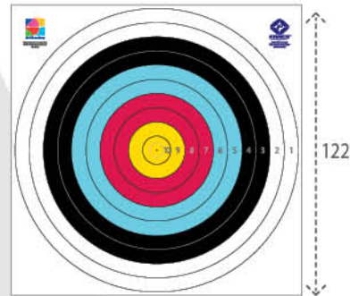
PT 001F OUTDOOR 122cm Target Face Range : 90m / 70m / 60m Mark dimension : 122cm X 122cm Total dimension : 125cm X 125cm (width/length)
