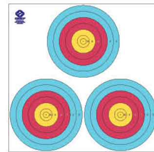
PT 007A3 OUTDOOR Triangular Target face(6Line) Range : 50m Mark dimension : (48cm-Center X 3Target) Total dimension : 99cm X 98.5cm (width/length)
