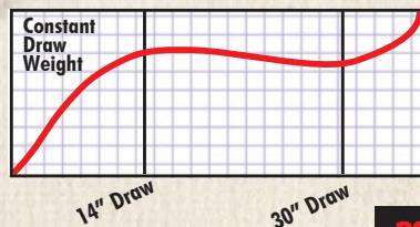
DISCOVERY™ 2 DRAW PROFILE
