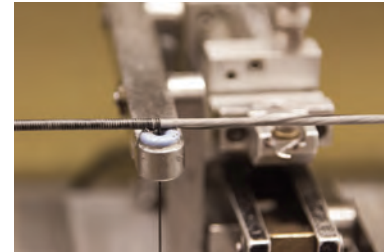
The LiveWire™ machine then wraps the string under full load, serving throughout the entire process at tensions previously impossible to achieve.
