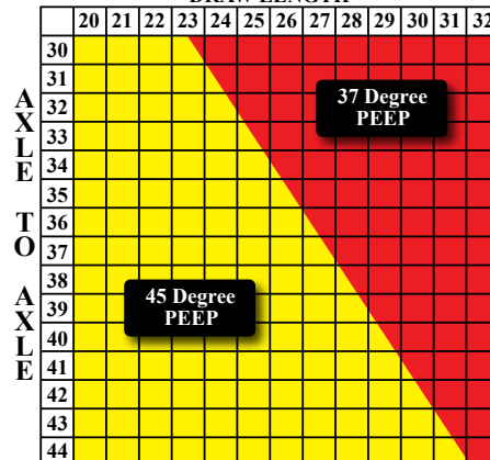
6" BRACE HEIGHT DRAW LENGTH
