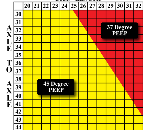
8" BRACE HEIGHT DRAW LENGTH
