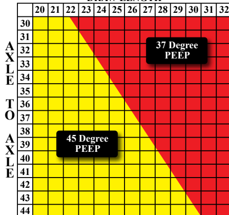
5" BRACE HEIGHT DRAW LENGTH
